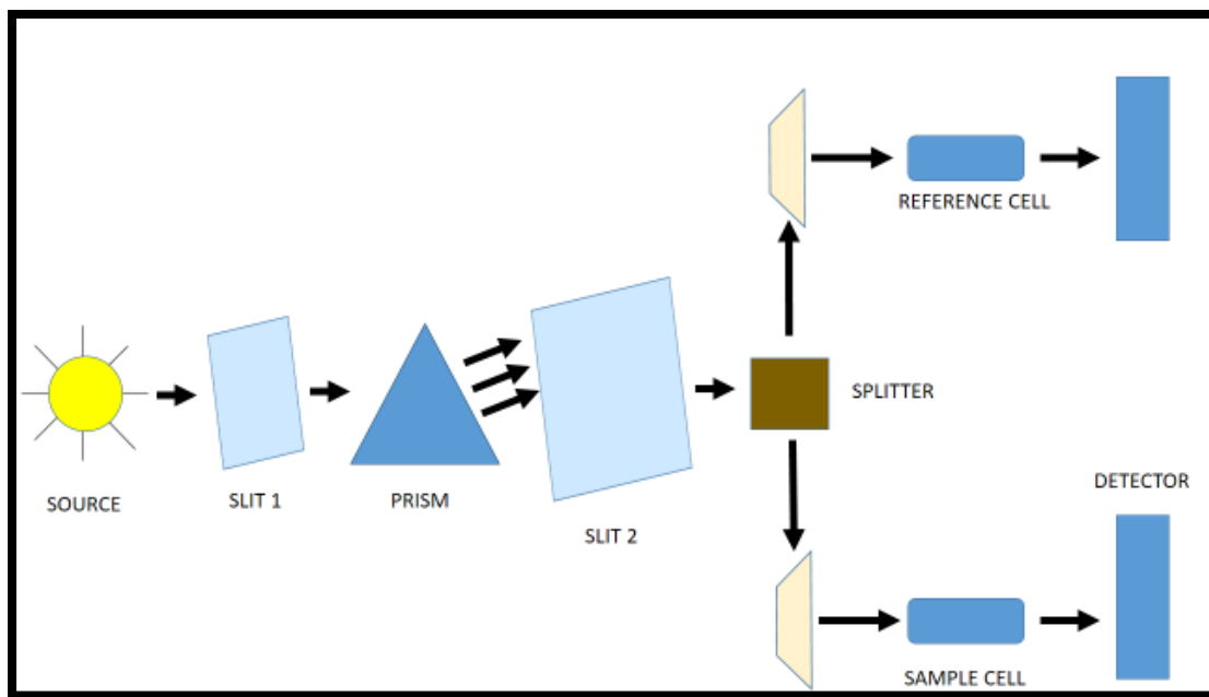
Schematic of Spectrometer
